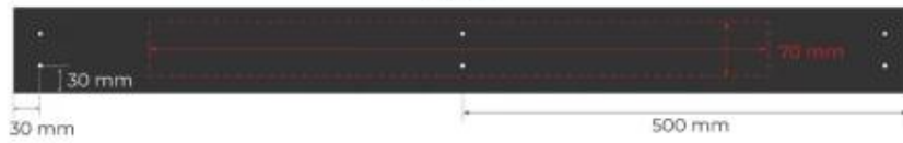
Top view with fixing points and burner cutout with lip in bottom plate 770 mm
